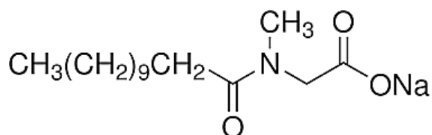
Figure 4. Structure and formula of NLS [172]
